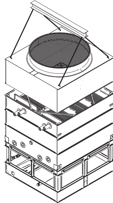
Figure 19 - Mating Fan Section to Coil/Basin
