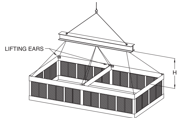
Figure 4 - Basin Section 24' to 40' long
