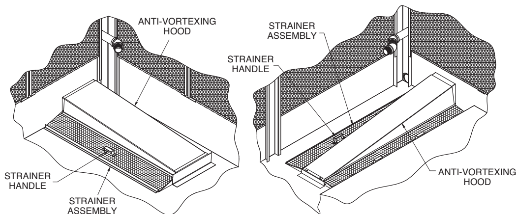
Figure 34 - Strainer Location
