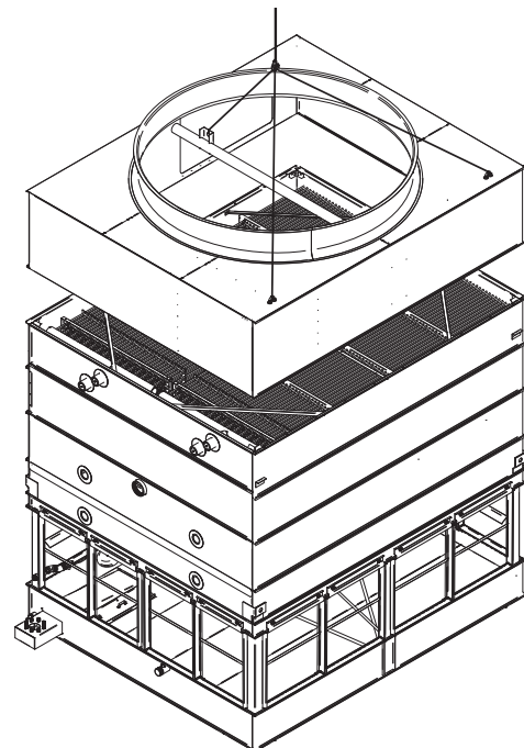
Figure 20 - Mating Fan Section to Coil/Basin
