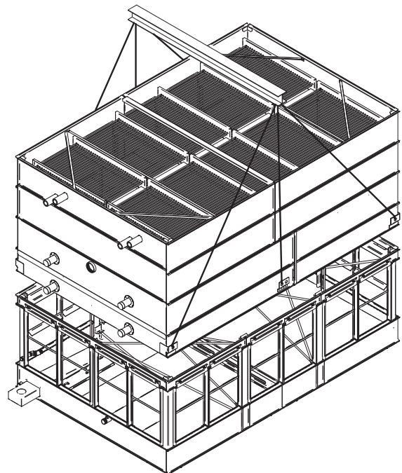
Figure 18 - Mating Upper Section to Basin Section
